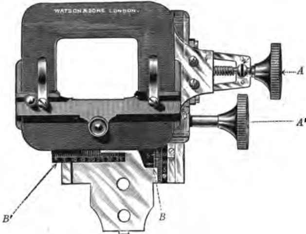
FIG. 45.—Mechanical stage.
